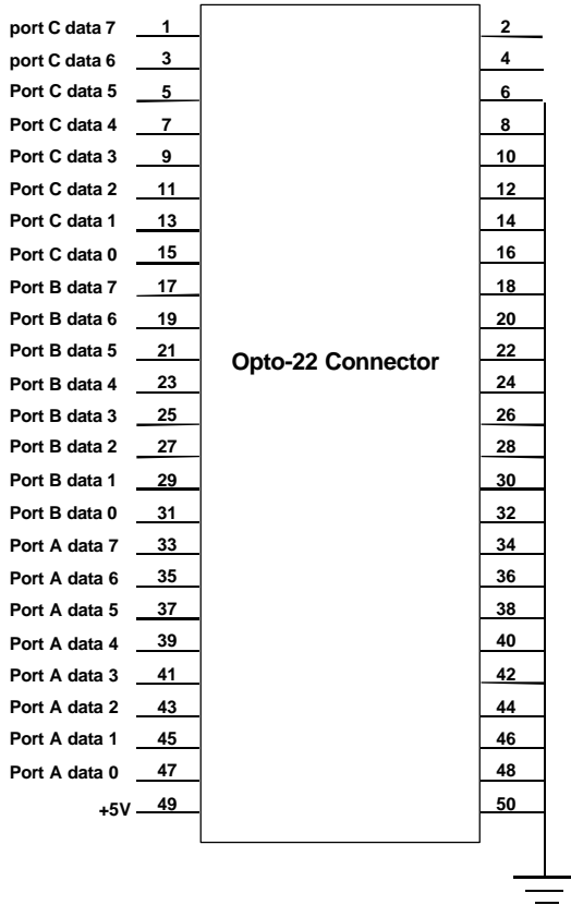
CN6 pin definition
