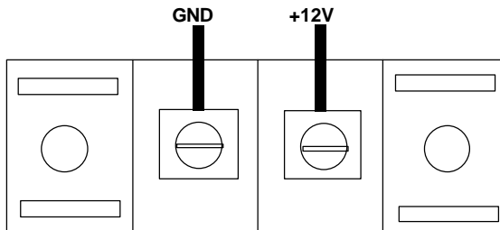
CN5 Connection
