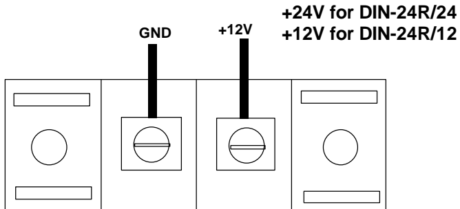
CN5 connection
