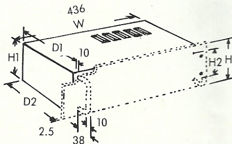
FRONT PANEL 1U
