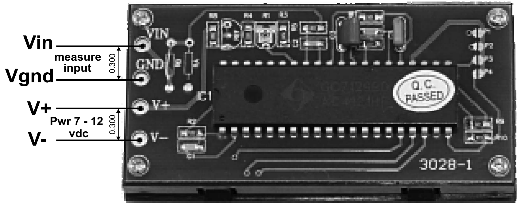
Meter Rear View
