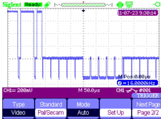
Figure 2-45 Video Trigger
