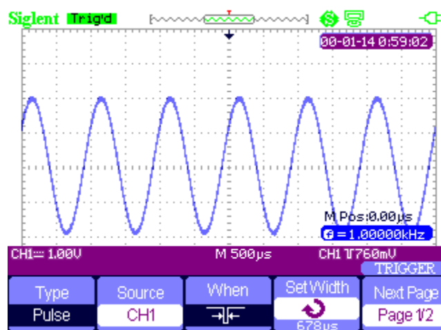
Figure 2-42 Pulse Trigger
