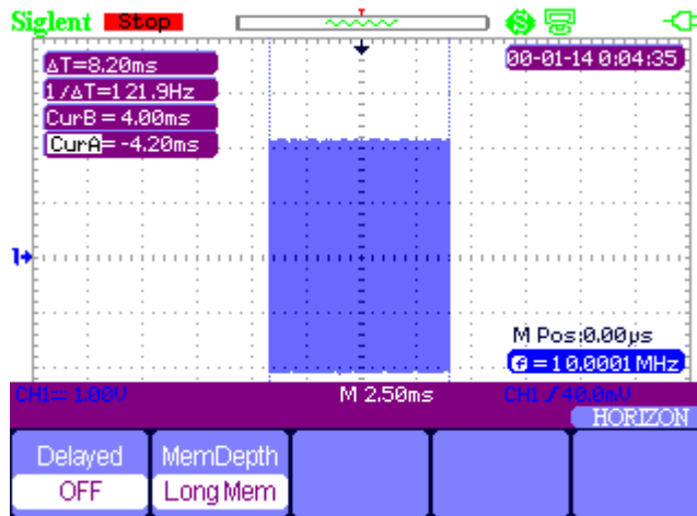
Figure 2-23 Long Memory
