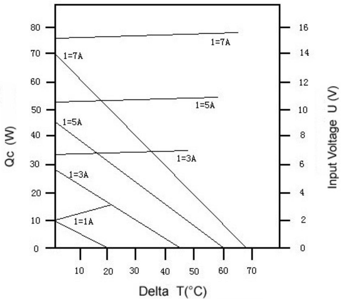
TEC1-12707 Characteristic of Input and Output
