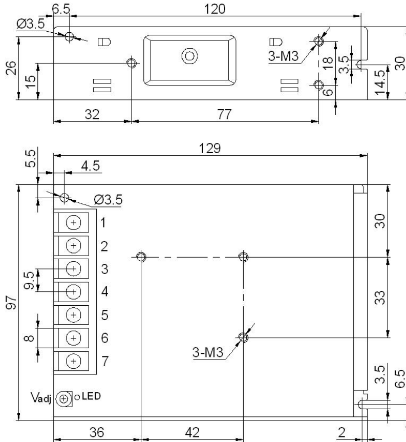
Terminal Pin No. Assignment 接线端子排布:
